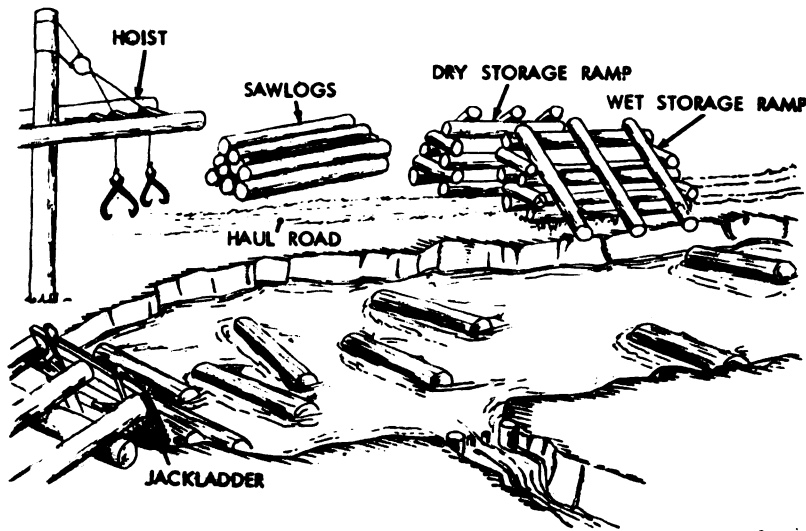
Figure 7-20. Wet-storage facility.
